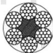
6×19W + FC
