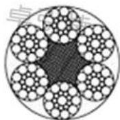
6×19S + FC
